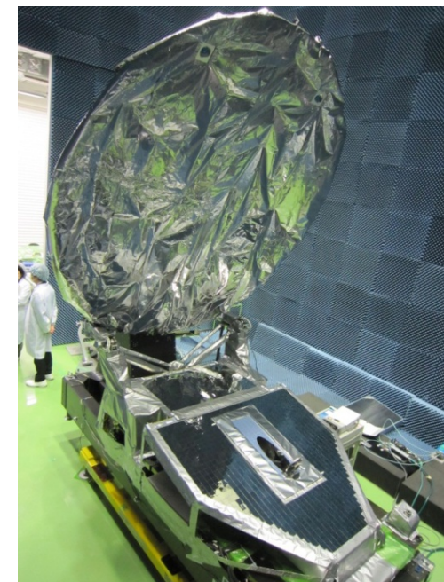
EarthCARE/CPRの外観
