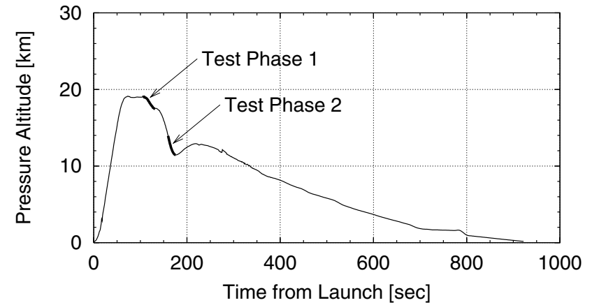
Fig. 2: Flight Altitude
