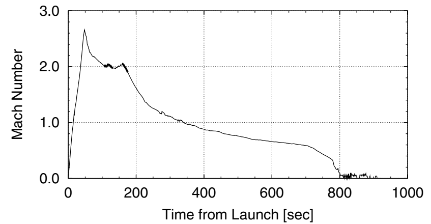
Fig. 3: Flight Speed
