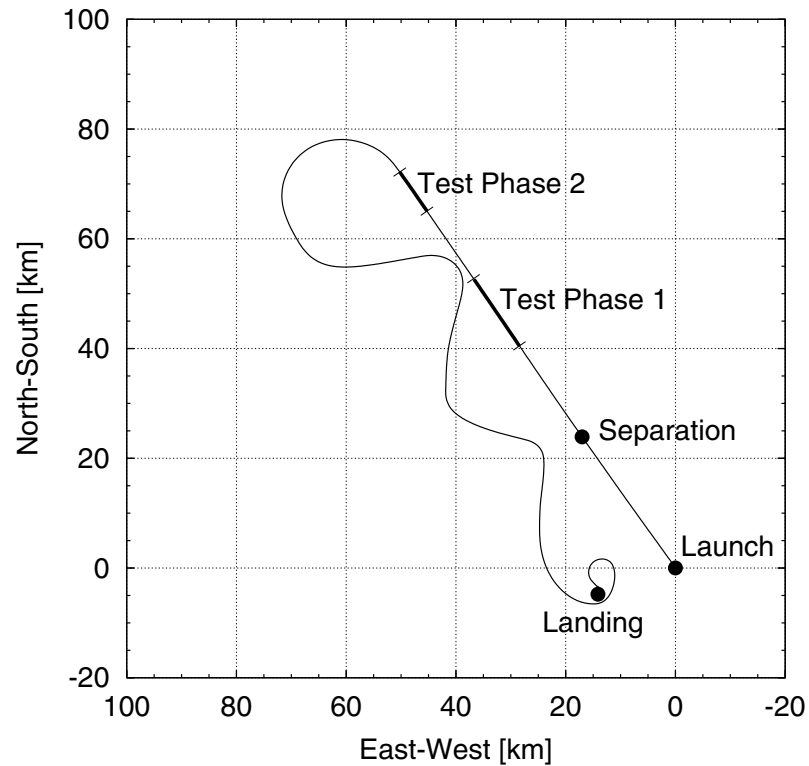
Fig. 1: Flight Trajectory
