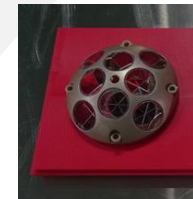
LRA(Laser Retroreflector Array) provided by NASA. The LRA consists of an array of multiple mirrors that are retroreflective and reflect light back in the direction of origin. Mass is approximately 21g.
